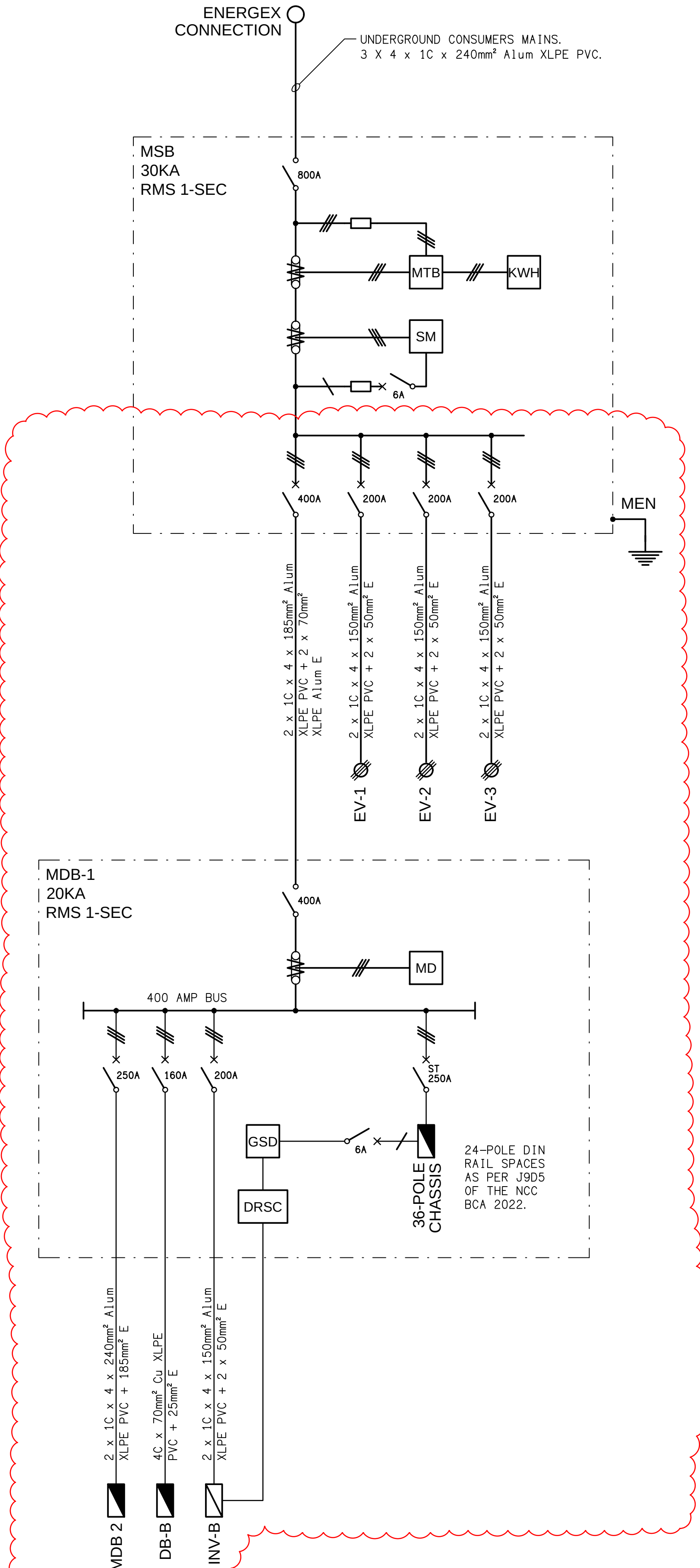
SCHEMATIC MSB CONFIGURATION NOT TO SCALE
