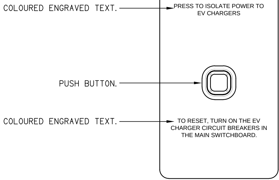
DETAIL ELECTRIC VEHICLE CHARGING ISOLATION SWITCH (CIS) NOT TO SCALE
